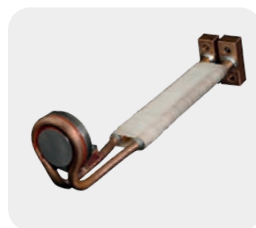
Round front focus coil (order no. 09-119-01)
