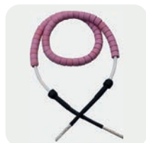
FLEXI ceramic coil (order no. 80-257-01)
