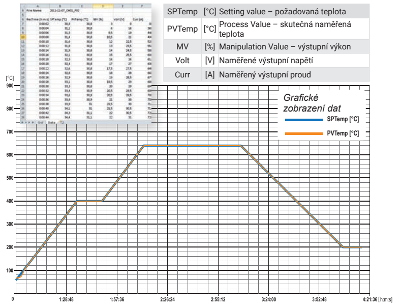
Output from the built-in recorder of the inverter DHC 6510R
