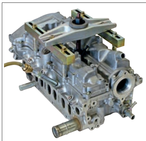
KL-0186-14 KA Injector Nozzle Puller Set Like KL-0186-14 EA , but in a Plastic Suitcase
