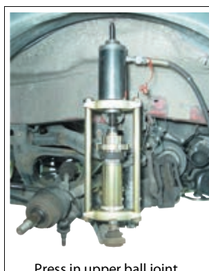
Press in upper ball joint
