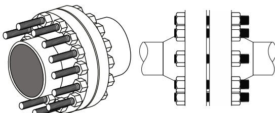
50% Bolt Tensioning
