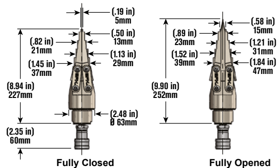
FLS15-ST Spreader
