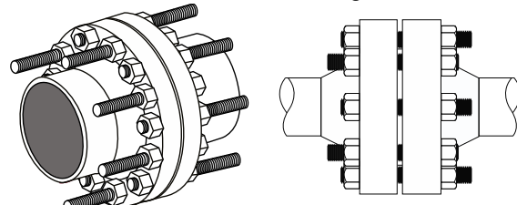
100% Bolt Tensioning
