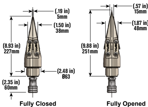
FLS15 Spreader
