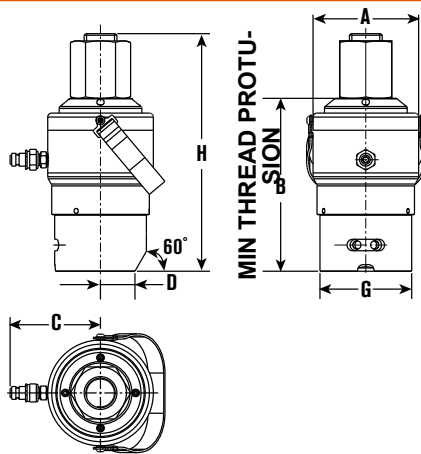
Manual Nut Rotation Version
