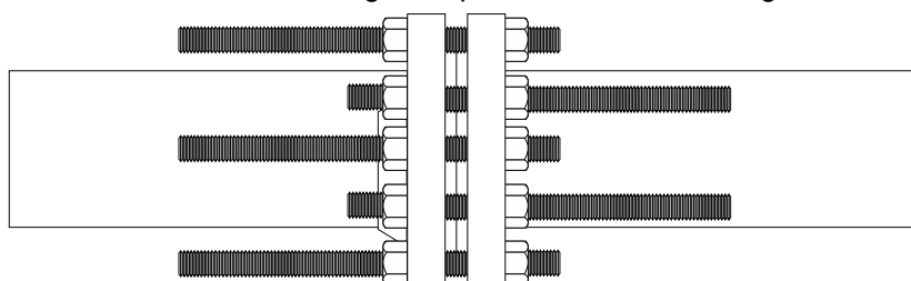
100% Tensioning Set-up for Subsea Tensioning
