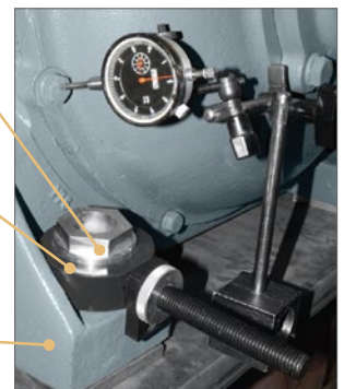
Eccentric socket
