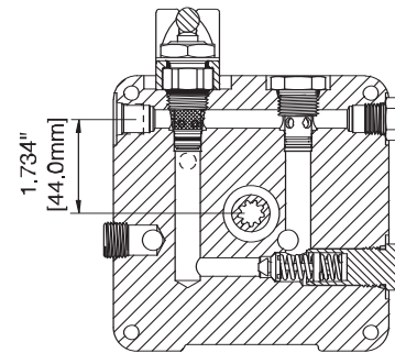
ENDHEAD SECTION
