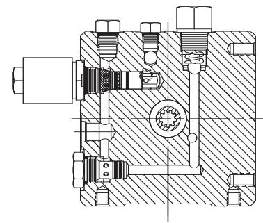
ENDHEAD SECTION
