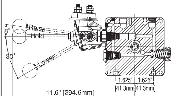
ENDHEAD SECTION
