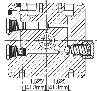
ENDHEAD SECTION
