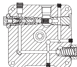
ENDHEAD SECTION
