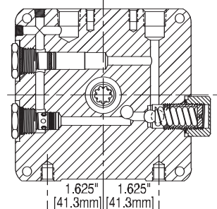
ENDHEAD SECTION
