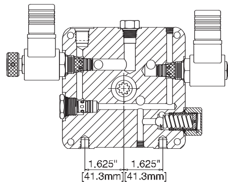
ENDHEAD SECTION
