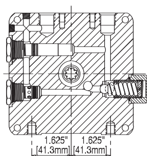
ENDHEAD SECTION
