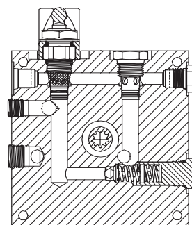
ENDHEAD SECTION
