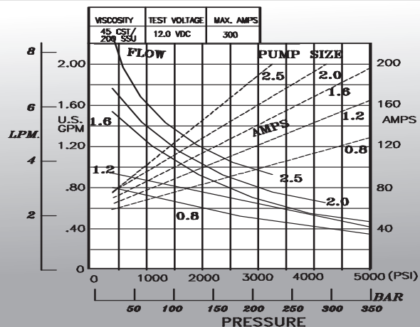
KMD8 12V Flow/Amp vs. Pressure Curve
